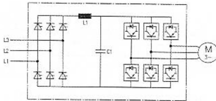
Fig. 2. Basic structure of a frequency converter with voltage inverter
