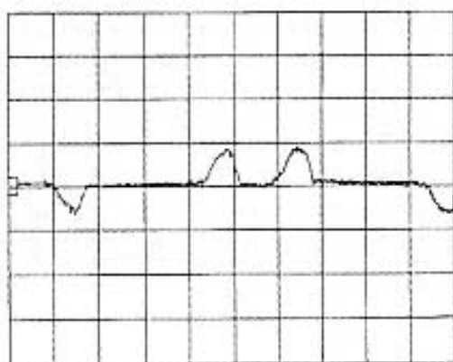
Fig. 4. Mains current with L_1 choke
