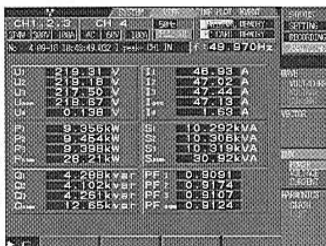
Fig. 9. Power taken up from the mains
