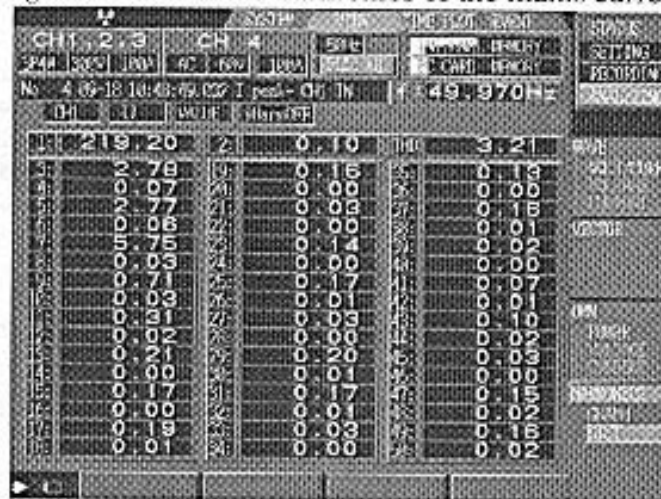
Fig. 7. Values of the harmonics of the mains current
