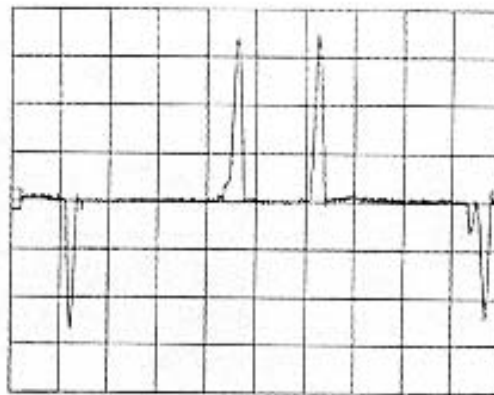
Fig. 3. Mains current without L_1 choke
