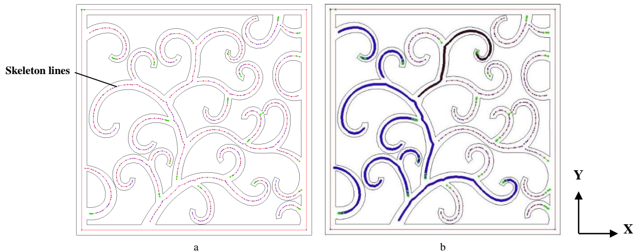
Fig. 6. (a) A designed architectural carve pattern with complete skeleton lines; (b) Tool paths planning (black stripe: current tool path being planned; blue stripes: tool paths that have been planned).
